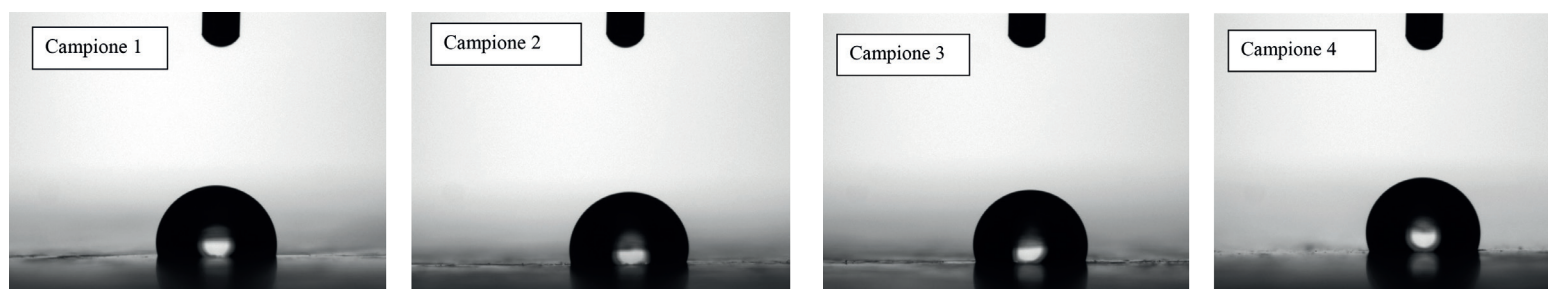
FIG. 1 Contact angle measurements images of four samples
